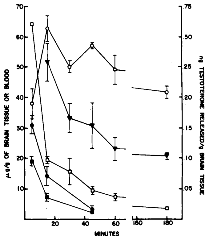
Figure 1—Concentrations against time for the testosterone-17-nicotinate-N-methyl cation, calculated as iodide, in brain (O) and in blood (□) and concentration of released testosterone (ng/g) in brain (♥) following administration of the corresponding dihydropyridine derivative I. Concentrations of testosterone in brain (●) and blood (■) following administration of testosterone are also included. Bars represent the standard errors.
